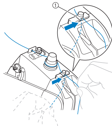
① Guide plate
