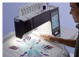
Large 360mm x 350mm Embroidery Field
